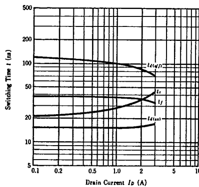
SWITCHING CHARACTERISTICS
