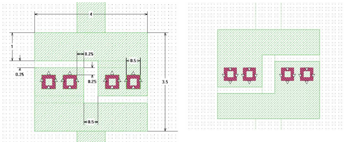
Fig. 2.7c. 434 MHz cross tapped loop antenna. Zoomed picture of antenna RF feeding points on the top layer and DC feeding on bottom layer (dimensions in mm).
