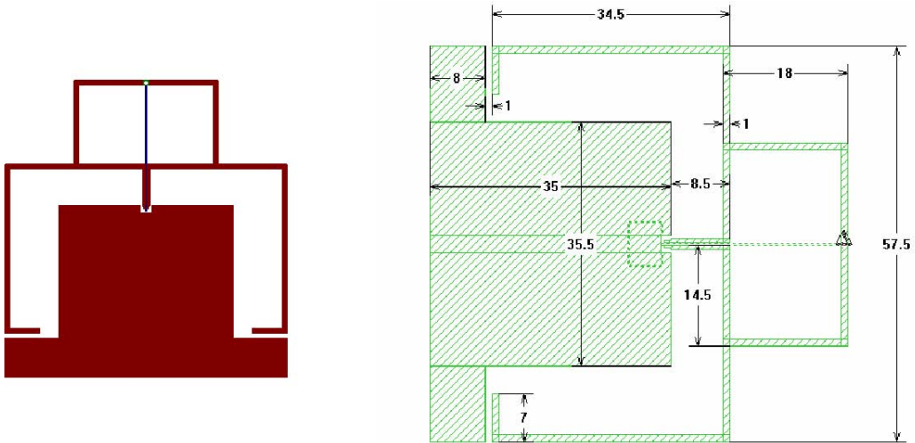
Fig. 2.6a. 868 MHz BIFA antenna. Top layer (dimensions in mm).
