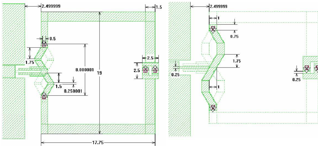
Fig. 2.4b. 915-868 MHz dual band cross tapped loop antenna, "big" type: top layer and bottom layer (top v. (dimensions in mm).
