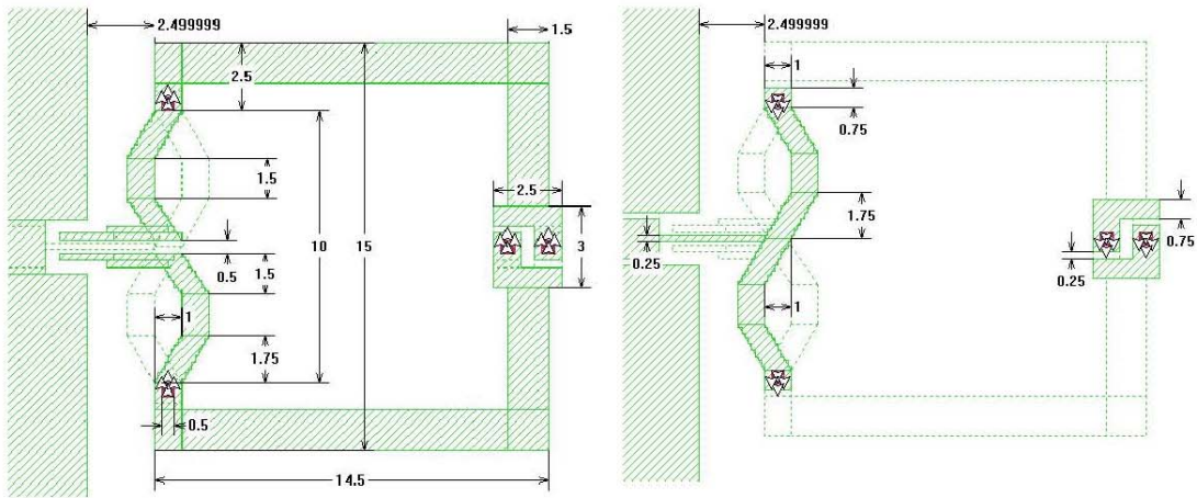
Fig. 2.3b. 915-868 MHz dual band cross tapped loop antenna, “small” type: top and bottom layer (top view) (dimensions in mm).
