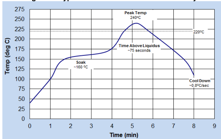
Figure 2: Typical Soak Reflow Profile for SAC Alloys
